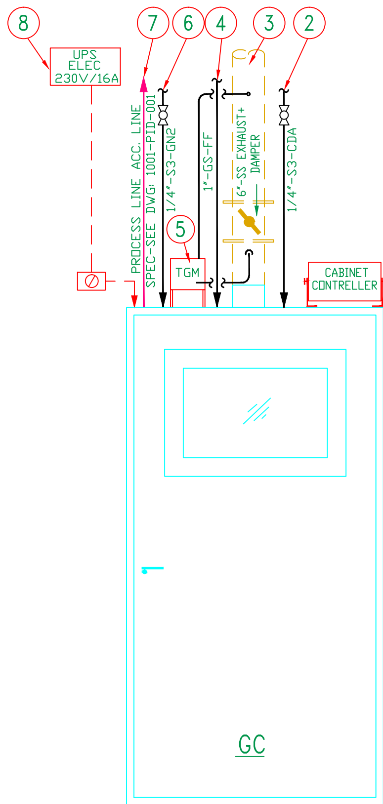
TYPICAL 2 CYL. CABINET UTILITIES SUPPLY (1 PROCESS + 1 PURGE)
